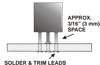
Figure 8. Installing Transistors.
