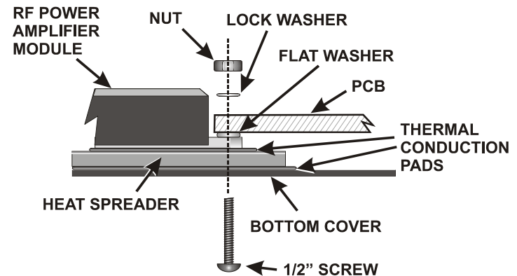
Figure 42. RF Amplifier Module Mounting Hardware.
