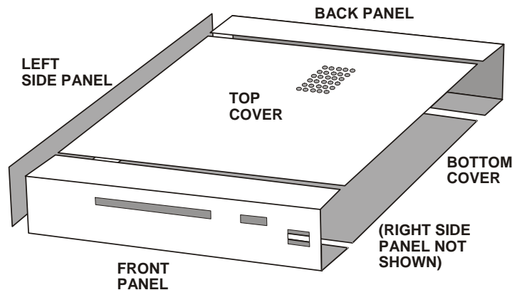
Figure 1. XV Transverter Modular Cabinet Parts.
