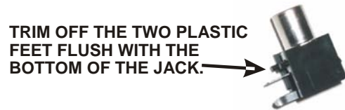
Figure 24. Preparing the RCA Jacks for Installation.
