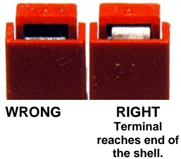
Figure 27. Verify Contact is Fully Inserted.
