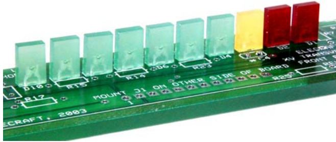
Figure 11. Power LEDs Installed on Front Panel PCB.
