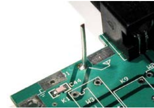
Figure 29. PCB Antenna Connection.
