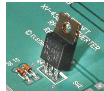
Figure 22. Installing Transistor Q4.
