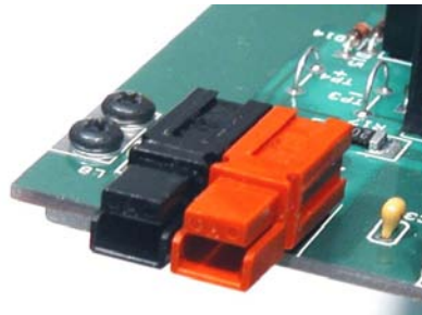
Figure 28. Orienting J7 on the RF PCB.
