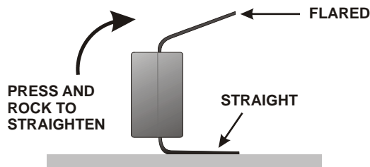
Figure 43. Straightening IC Pins.
