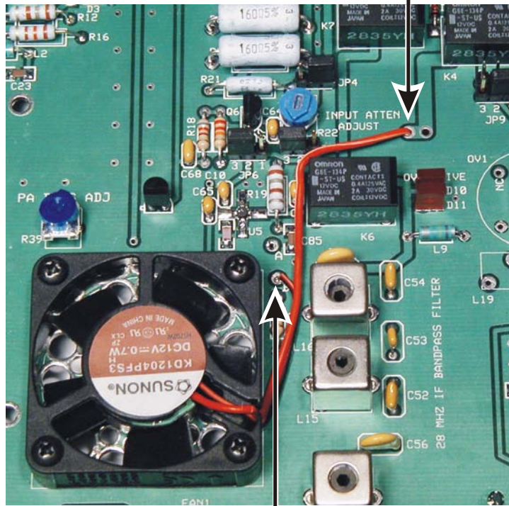
BLACK WIRE SOLDERED TO PAD B. Figure 37. Installing Fan.
