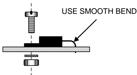
Figure 19. Installing Voltage Regulator U4.
