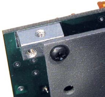
Figure 41. Bottom Cover Attached to a 2-D Fastener.
