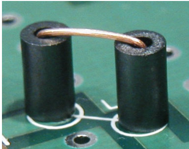
Figure 20. Installing L7.
