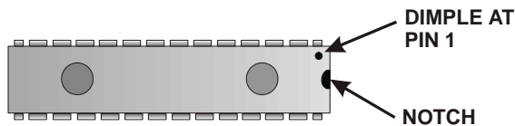
Figure 44. IC Orientation.
